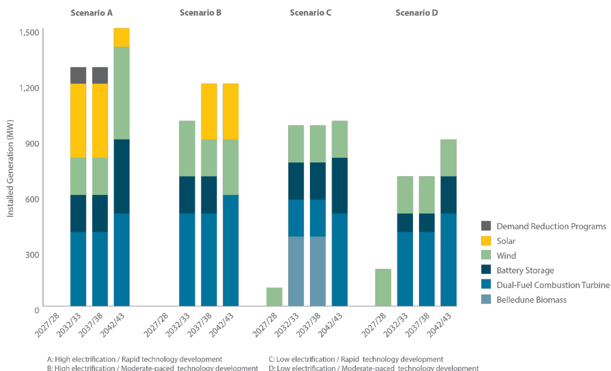
Figure 12.1: Mactaquac Replacement Generation Capacity
