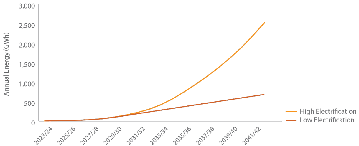
Figure 7.8: Projections of Electric Vehicle Annual Energy Requirements
