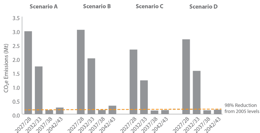
Figure 12.8: GHG Emissions – No SMR Scenarios
