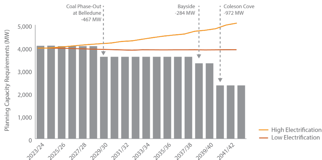
Figure 9.3: Load & Resource Review 56
