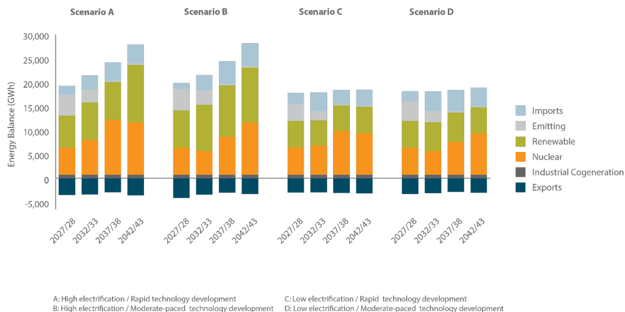
Figure 11.8: Energy Balance by Scenario
